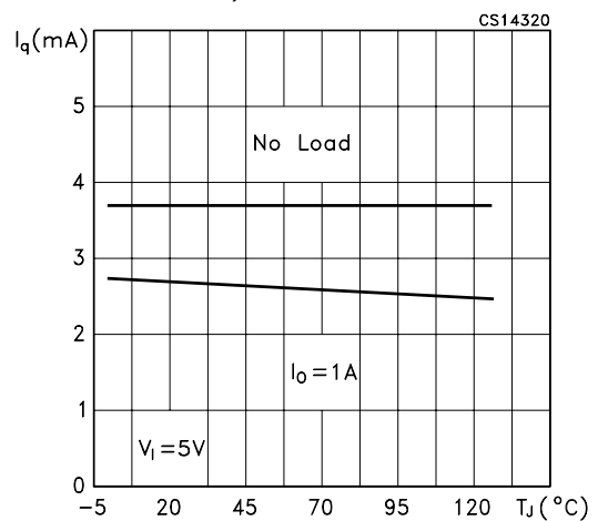
Figure 17 : Quiescent Current vs Temperature (Fixed/ADJ Version)
